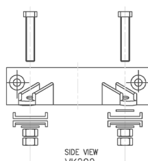
SIDE VIEW VK202
