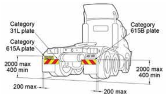
PRIME MOVER WITH 615A AND 615B STRIPS AND 31L PLATES
