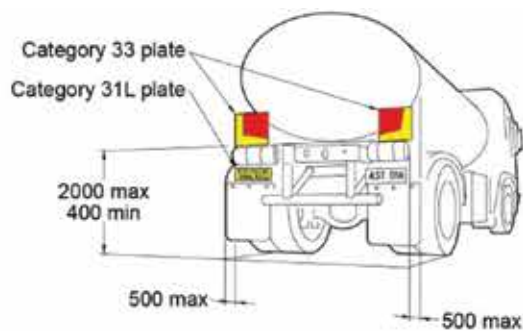
ROAD TANK VEHICLE WITH CATEGORY 33 PLATES
